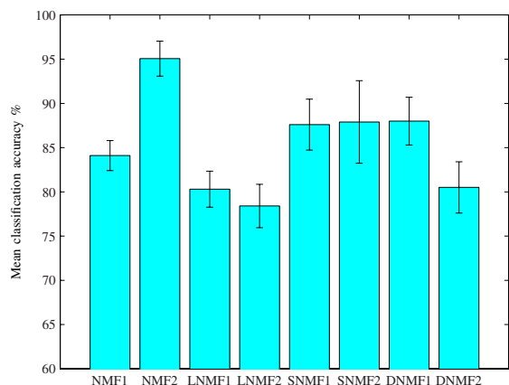
Fig. 1. Classification accuracy of NMF algorithms, where 1/2 refers to the feature vector used
