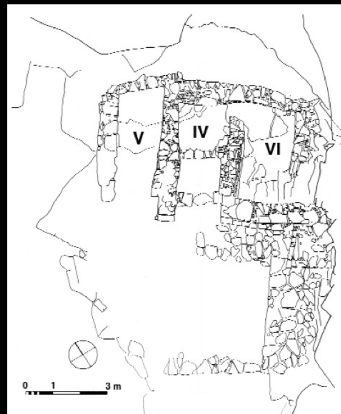
Fig. 5.16: Plan of Tomb IV/V/VI at Mochlos (after Soles 1992: 52 Fig. 20, courtesy of the Trustees of the American School of Classical Studies at Athens).
