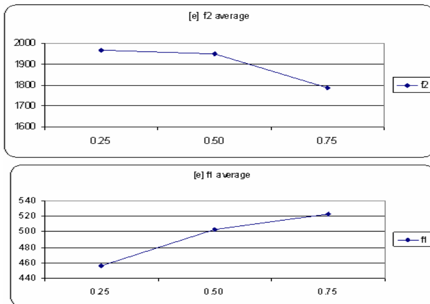
Figure 6. Movement of F1 (bottom) and F2 (top) from the values typical for [i] to the values typical for [e] in [je] sequences (average from 10 tokens).
